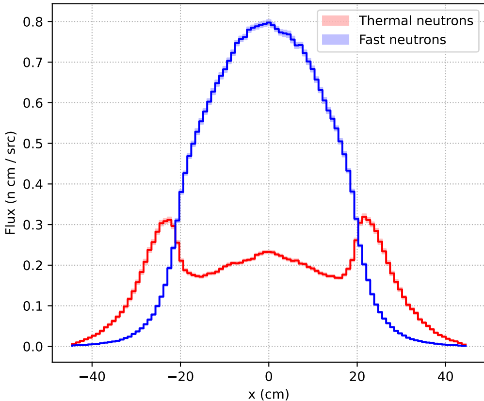
1D Flux Profile Along X - energy components
